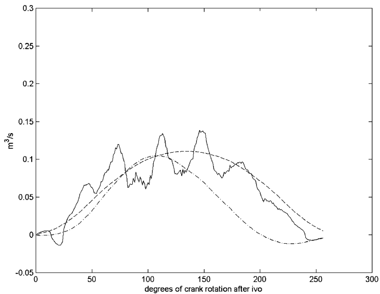
Fig. 13. Single cylinder Formula 1 engine. Calculated and measured volume flow rates, 7000 rev/min wide open throttle. Measured (solid line), calculated from Eq. (2) (chain dotted line), calculated by scaling the open area under the lifting valve (dashed line).
